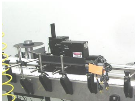
AutoLabe 110 applicator with wrap unit, photo electric sensor.
